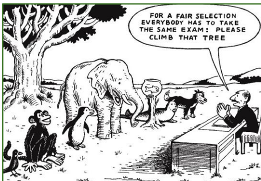
Abb. 4: Quelle: https://mathcoachblog.com
